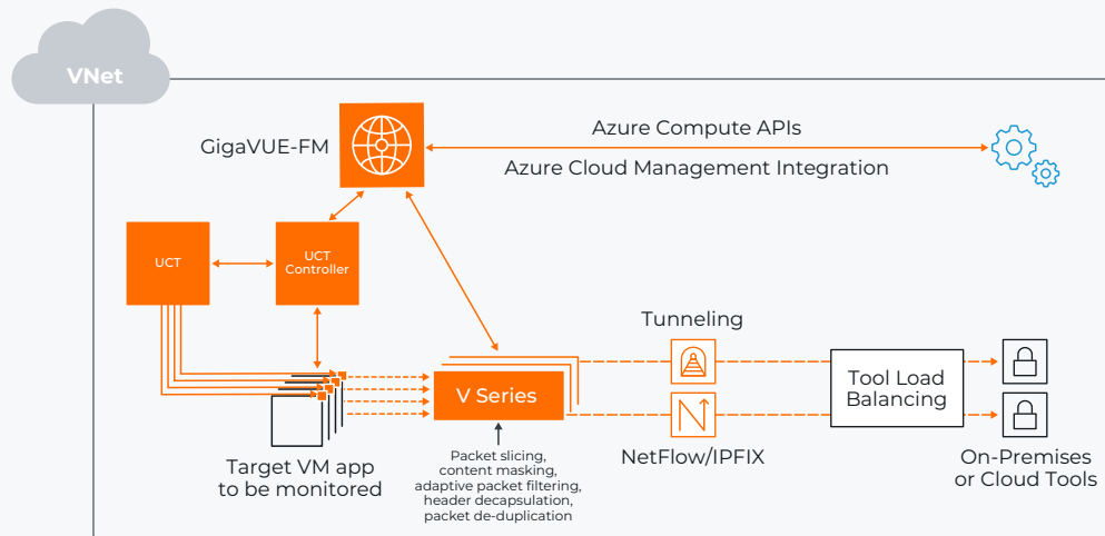
Figure 3. GigaVUE Cloud Suite for Azure is composed of GigaVUE V Series for optimization, transformation, and brokering, as well as GigaVUE-FM for management. For access to workload traffic, GigaVUE Cloud Suite also includes the components UCT and UCT Controller, which are optional, but may be preferred in situations where free workload-level visibility is preferred over paid Azure services.
